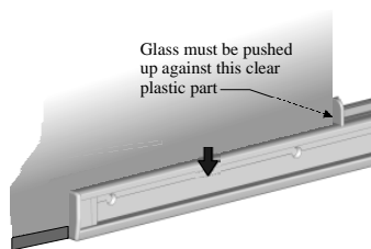
Bottom Rail-Inside View Fig. 14
